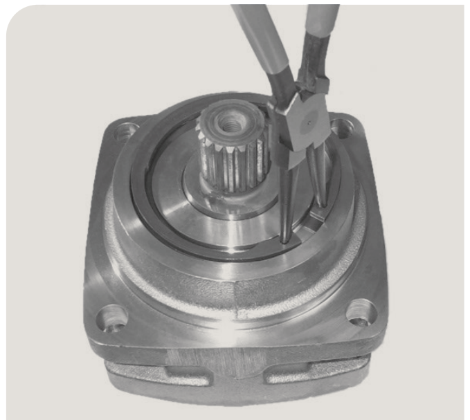
8. Assemble the retaining ring.
