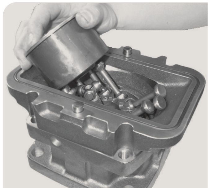
16. Assemble the cylinder barrel.
