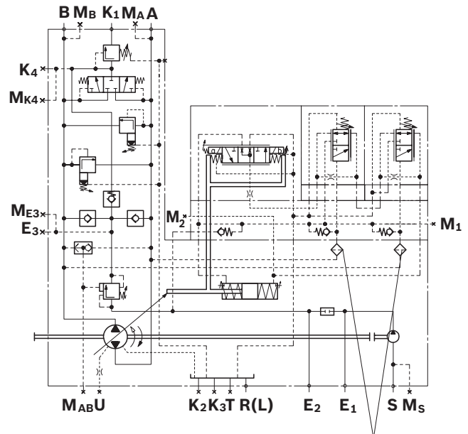
Control fluid filter for HD and EP (nominal sizes 500 and 750)
